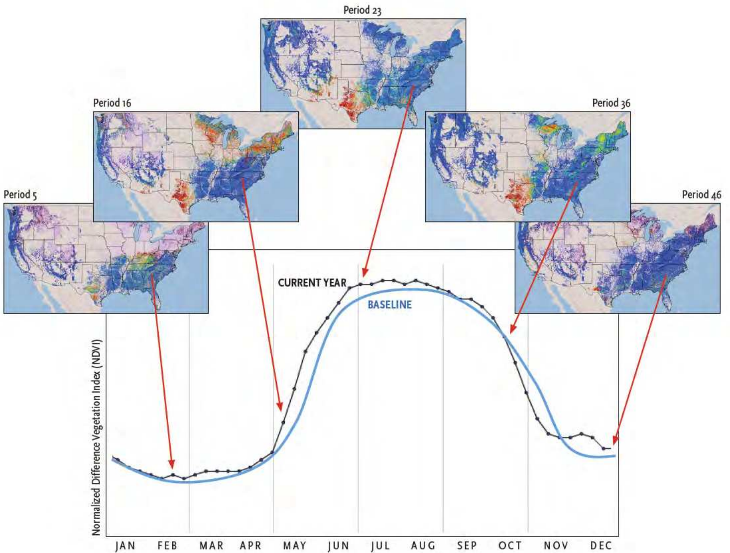
Figure 3b—An annual NDVI curve for one site in North Carolina compared to a hypothetical baseline curve. Every year, forty-six change maps are produced for each combination of current conditions with the 1, 3, and all year baselines which provide different seasonal expectations of normal.
