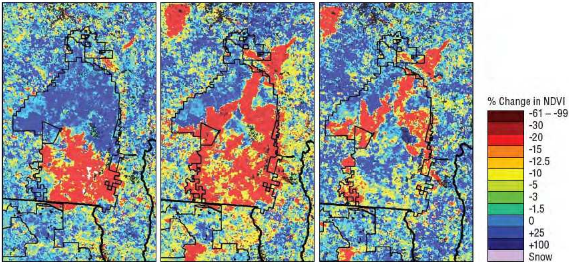
Figure 13—Georgia’s Okefenokee Swamp National Wildlife Refuge near the Georgia-Florida State line burned in 2007 and again in 2011. This rapid recovery of fuels reflects the importance of sprouting vegetation. This image sequence from the summer of 2011 illustrates the vegetative resilience in the region. By June 17, wildfire, as shown in red, had spread northward through about half of the Refuge (left). By July 19 (center), fire had progressed north, and a new fire became evident northwest of the Refuge. By August 20 (right), vegetation in the area that had burned in May and June had recovered to the long-term baseline NDVI, as shown in blue. This fire burned over 300,000 acres.
