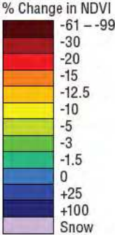
Figure 6—Immediately prior to a hard mid-September frost in 2011, the forests of the Upper Midwest experienced fall much like they did during 2010 (top; ending September 13). However, in the weeks following, a strong forest change anomaly developed over northeastern Minnesota, northern Wisconsin, and the upper peninsula of Michigan (bottom; ending October 15). The dark patch in extreme northeastern Minnesota (indicated by the black arrow) is the Pagami Creek wildfire that made a major run shortly after the NDVI values were collected for the top image. See figure 14 for more detail on this wildfire. The photograph on the left shows the effects of a spring frost on greenup. ForWarn captures frost effects in both spring and fall.
